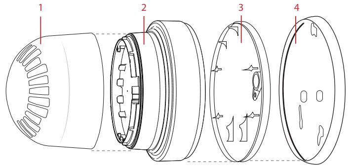
1 Sounder / visual indicator, 2 Wireless module, 3 Battery retaining plate, 4 Mounting plate
