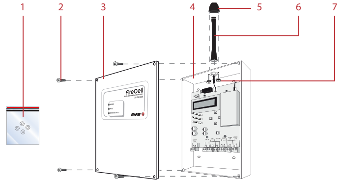
1 4x washers, 2 4x lid screws, 3 RNC lid, 4 RNC back box, 5 Anti tamper shroud, 6 RNC aerial, 7 2x thumb nuts
